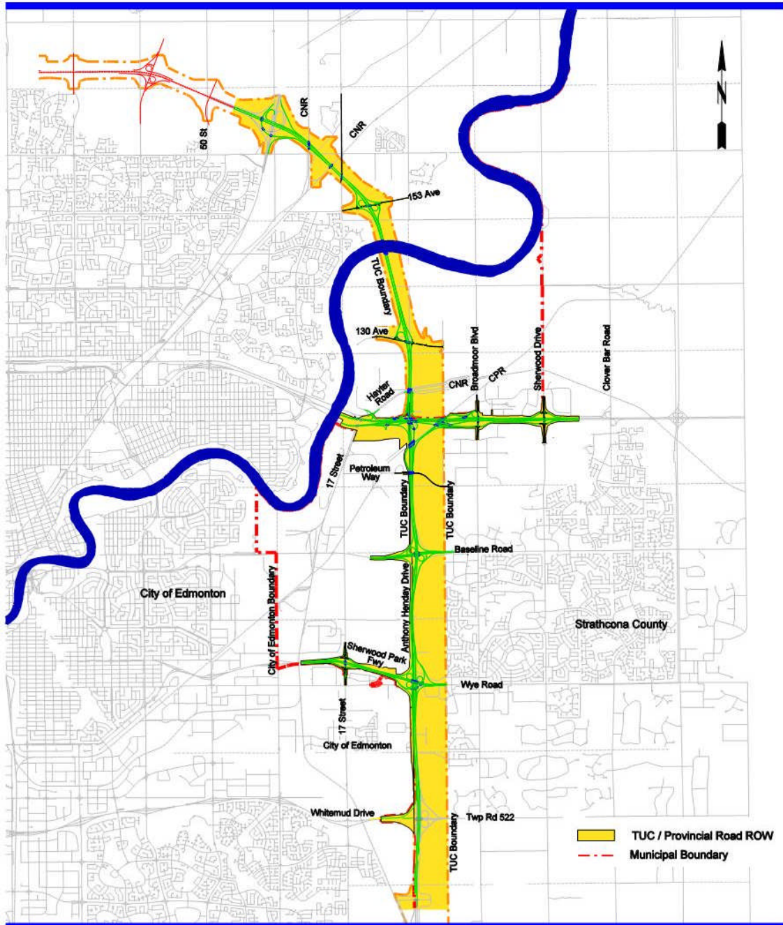
Figure 2: Northeast Anthony Henday Drive Stage 1
