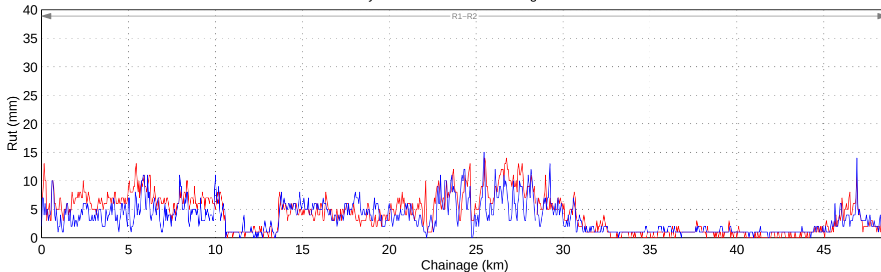
Hwy 3:10 Wheel Path Rut – Right Lane
