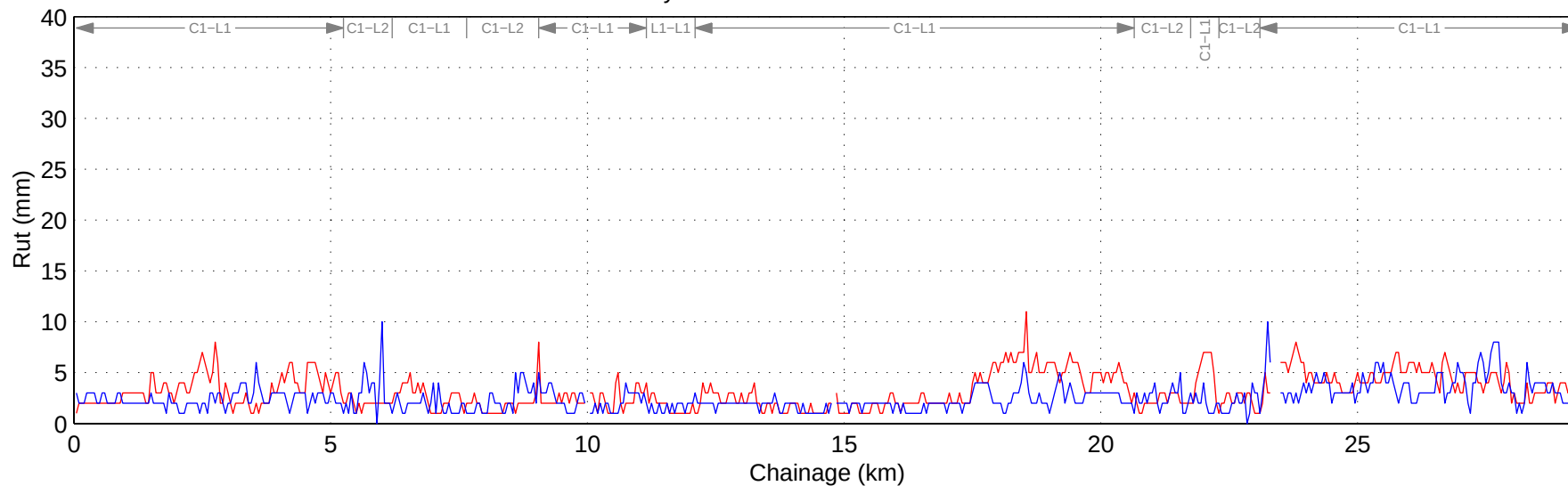
Hwy 3:04 Wheel Path Rut – Right Lane
