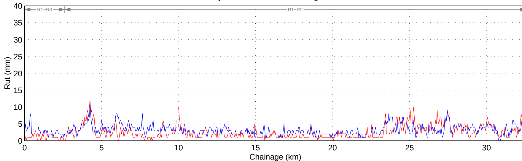
Hwy 1:02 Wheel Path Rut – Right Lane
