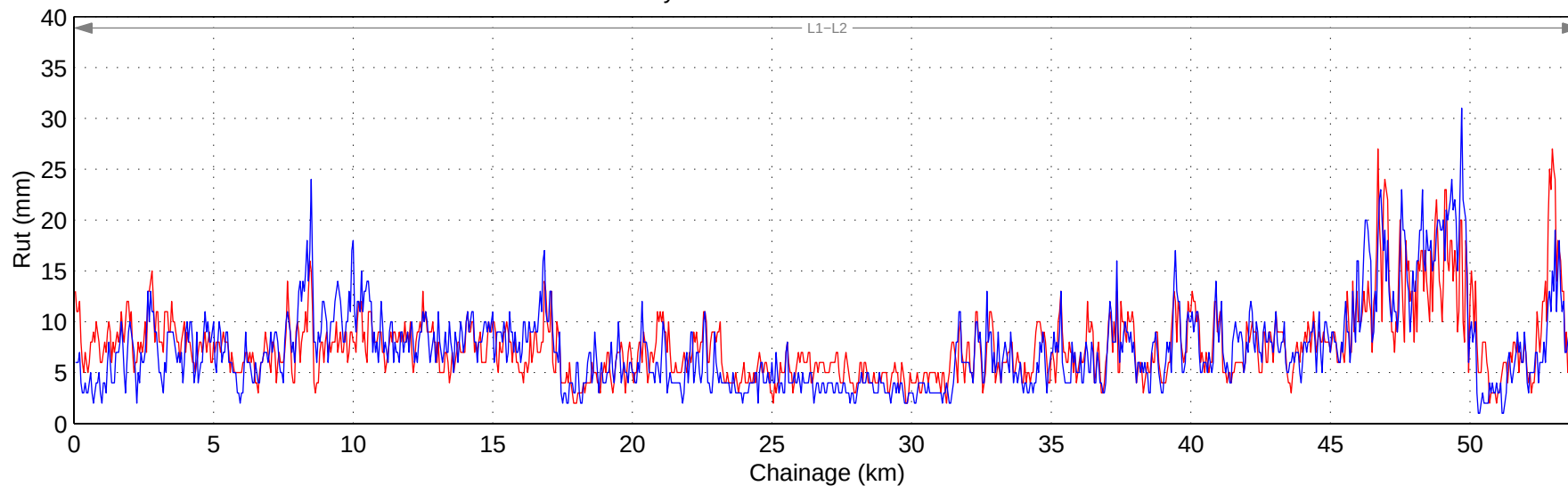
Hwy 1:20 Wheel Path Rut – Right Lane
